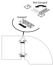
Ganging Bracket
