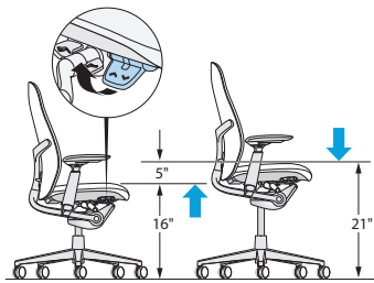
Fully Retracted
