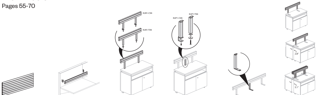
Rails and Mounting Slat, Wall Mount
