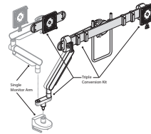
Accessories - Triple Conversion Kit
