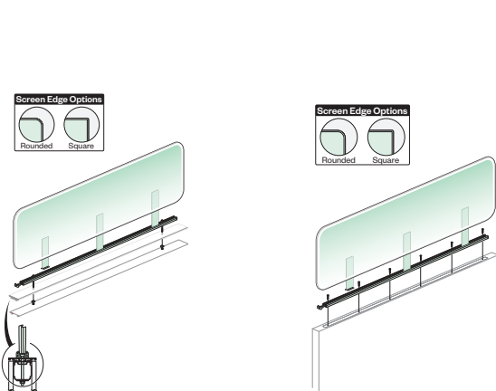
Compose Top Trim Channel Mount
