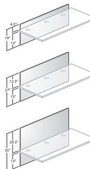
Modesty — Adaptable Convergent and Intuity Return Worksurfaces, and Height Adjustable Tables
