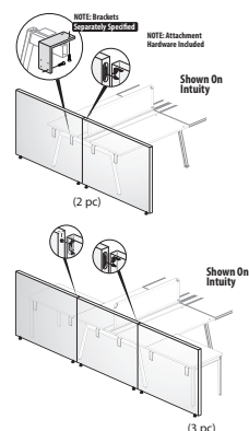
Intuity, Height Adjustable Benching, Adaptable Worksurfaces with 1, 2 or 3 Piece Universal Mount
