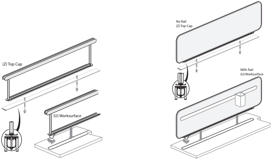
Accessory Frame - Open
