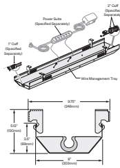
Dual-Hinged Cable Management Tray — Metal
