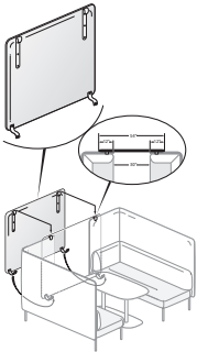
Connector Screen
