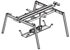
Angled Leg ZBRA-4848-SAGH (Shown with Utility Tray, 3- or 4-circuit power and access hatches) Class IN
