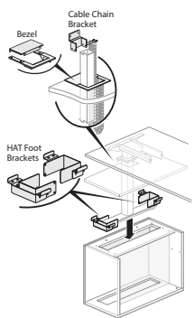
Hardware Kit — Height Adjustable Table Integration
