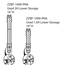
Compose Panel-to-Storage Bracket — C5 Be_Hold/Be_Hold Be and A Series Credenza
