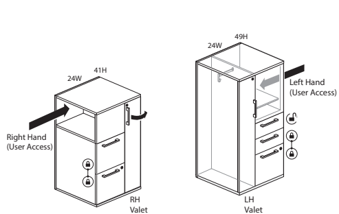
Personal Storage Towers - 24"W — Side Bookcase Upper Storage
