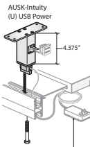
AUSK-Intuity (U) USB Power
