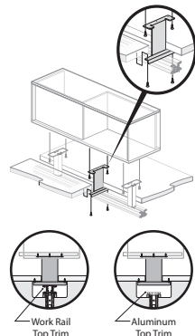
For use with Compose 26"(660mm) High Panel, Compose Connections and Compose Beam — Centered Single Panel Mount — Worksurface to Storage Bracket — Compose 26"(660mm) High Panel, Compose Connections and Compose Beam Mount
