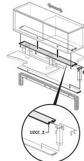
For use with Compose 26"(660mm) High Panel, Compose Connections and Compose Beam — Off-Modular Rail Mounting — Off-Modular Rail for mounting Compose to Be_Hold Upper Storage — Stanchion Mounted
