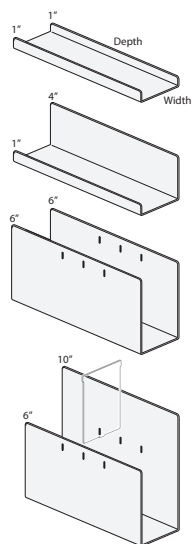
Belong Drawer Divider
